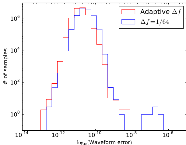
FIG. 8: Empirical interpolant approximation errors (the plus- and cross-polarizations only) when using an adaptive (red curve) and uniform (blue curve) frequency sampling. The adaptive sampling is used during the ROQ building procedure. To compute log-likelihoods with our ROQ rule we up-sample to a uniform frequency grid, and so this error (which constitutes the last in a series of approximations of the underlying model) is the most relevant for ROQ-accelerated inference studies. Results are shown for Case E only; other cases are qualitatively similar. Maximum upsampled EIM errors of 6 \times 10^{-9} , 1 \times 10^{-7} , 1 \times 10^{-5} , 7 \times 10^{-8} , 4 \times 10^{-7} and 1 \times 10^{-9} were computed for Cases A-F, respectively.
