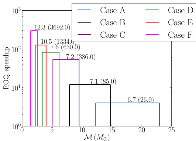
FIG. 10: Theoretical parameter estimation speedup (using the ROQ) for cases A-F in Table I. The speedup is calculated from the ratio L/(N_L + N_Q) , where L = (f_{\max} - f_{\min})/\Delta f is the number of quadrature points in the Full likelihood, N_L is the size of the linear basis and N_Q is the size of the quadratic basis. The sum N_L + N_Q is the number of points in the ROQ likelihood (11). The plot is annotated with the time (in hours) to compute 2 \times 10^7 ROQ (Full) likelihood evaluations, roughly the number of evaluations required for a typical PE analysis [5]. Our tests were performed using an Intel Xeon CPU with a 2.70GHz clock speed.
