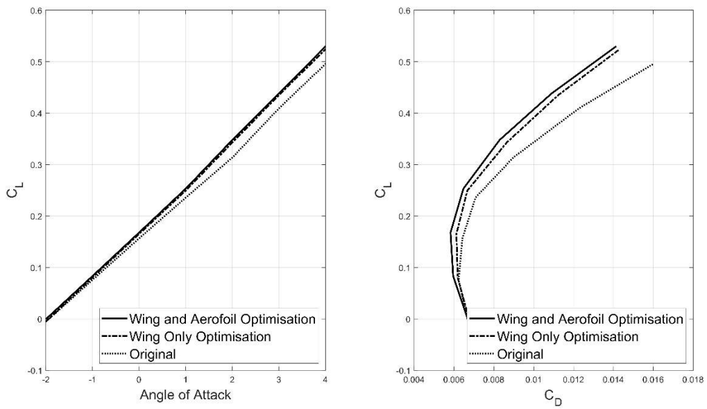
Figure 7. Lift curve and drag polar for the original wing, the redesigned wing using only wing planform parameters and the redesigned wing including airfoil shape optimisation
