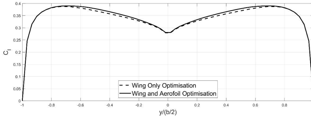
Figure 8. Local lift coefficient calculated using the corrected vortex ring strengths for an angle of attack of 2°.
