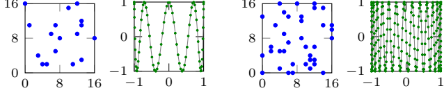
Fig. 4. Examples for arbitrarily chosen index sets I \subset \mathbb{N}_0^2 and corresponding rank-1 Chebyshev lattices \text{CL}(\mathbf{z}, M) fulfilling condition (7).
