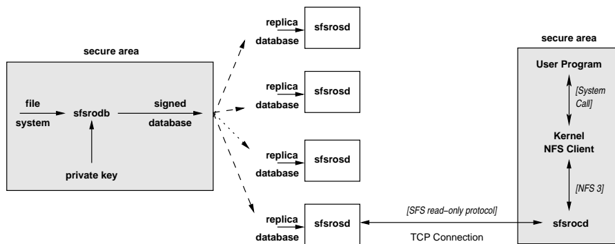
Fig. 1. The SFS read-only file system. Shaded boxes show the trusted computing base.
