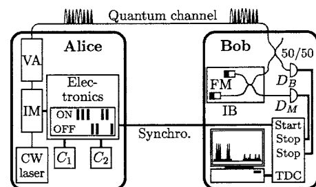
FIG. 3. Experimental setup.
