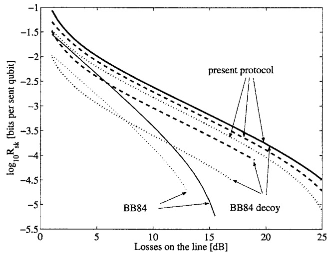
FIG. 2. An estimate of the secret key rates, Eq. (4), for the present protocol and for BB84 XY with and without decoy states, as a function of the losses on the line l ( t = 10^{-l/10} ). Parameters: \eta = 10\% , p_d = 10^{-3} , t_B = 1 , and f = 0.1 . Visibility: V = 1 (full lines, identical for the two first protocols), V = 0.9 (dashed lines), and V = 0.8 (dotted lines; R_{sk} = 0 for BB84 without decoy states).
