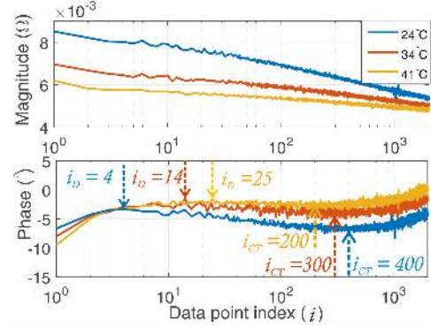
Fig. 9: Bode plot representation of the unfiltered impedance data obtained with ternary-sequence at 50% of SOC. Colored markings i_D represents the end of the diffusion part indices and i_{CT} the top of the semi-circle indices of the impedance at the corresponding temperature
