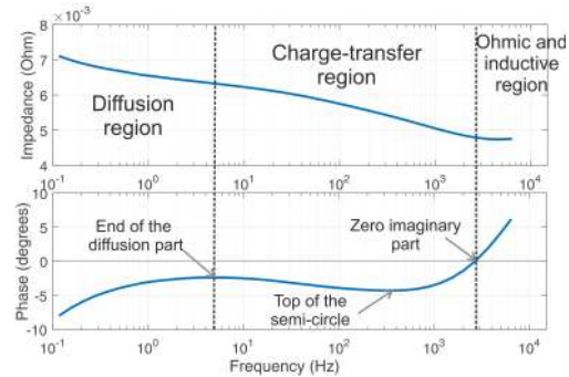
Fig. 2: Impedance Bode plot from LiFePO4 cell
