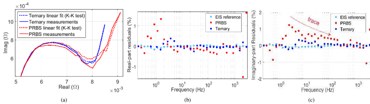
Fig. 11: a) Fitted impedances from the Kronig-Kramers test compared to the measured impedances at 25°C and 50% of SOC b) Real-part residuals from the Kronig-Kramers compliance test applied to impedance measurements at 25°C and 50% of SOC c) Imaginary-part residuals from the Kronig-Kramers compliance test applied to impedance measurements at 25°C and 50% of SOC
