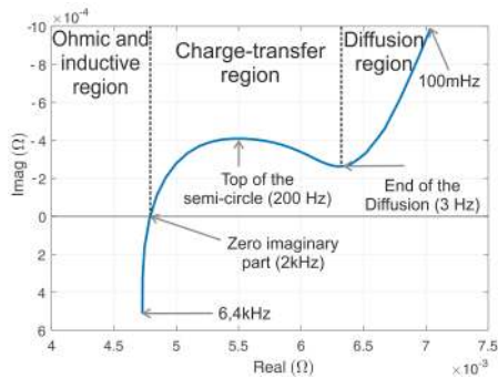
Fig. 1: Impedance Nyquist plot from LiFePO4 cell
