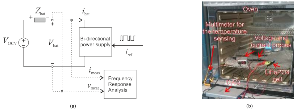
Fig. 6: a) Measurement setup configuration for the experiments b) Laboratory setup
