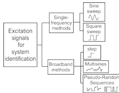
Fig. 4: Different excitation signals used for system identification
