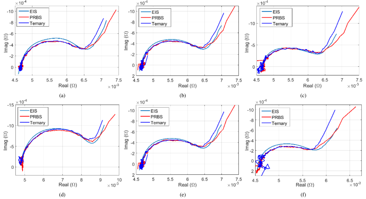
Fig. 10: Impedance Nyquist plot at 34°C and a) at 20% of SOC b) 50% at of SOC c) at 80% of SOC Impedance Nyquist plot at 50% of SOC and d) at 24°C e) at 34°C f) at 41°C
