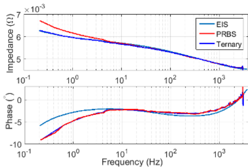
Fig. 12: Impedance Bode plot measured with different excitations at 41°C and 50% of SOC
