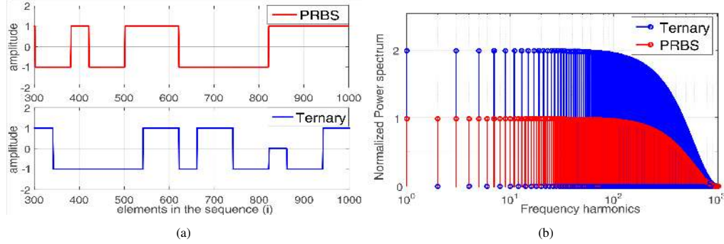
Fig. 5: a) time-domain characteristics of studied PRS signals b) Frequency-domain power spectrums of studied PRS signals
