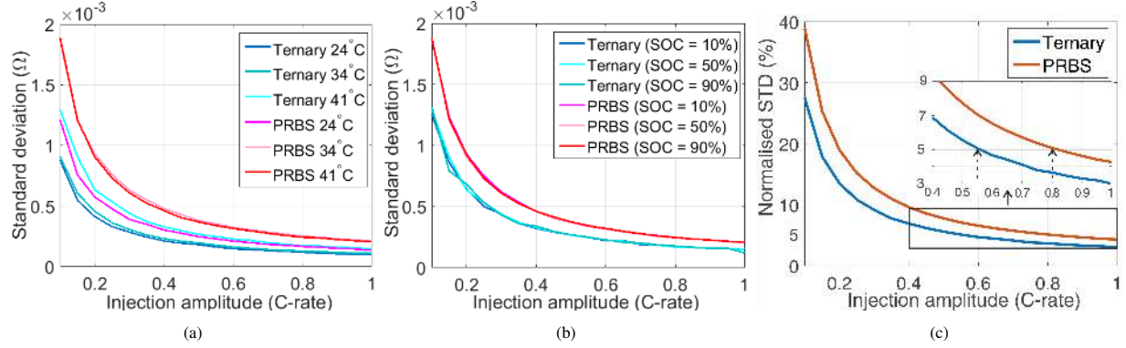
Fig. 7: a) Standard deviation of the impedance measurements as a function of injection amplitude at different temperatures at 50% of SOC b) Standard deviation of the impedance measurements as a function of injection amplitude at different SOC values at 41°C c) Normalised standard deviation of the ternary-sequence and PRBS as a function of injection amplitude at 50% of SOC and at 41°C
