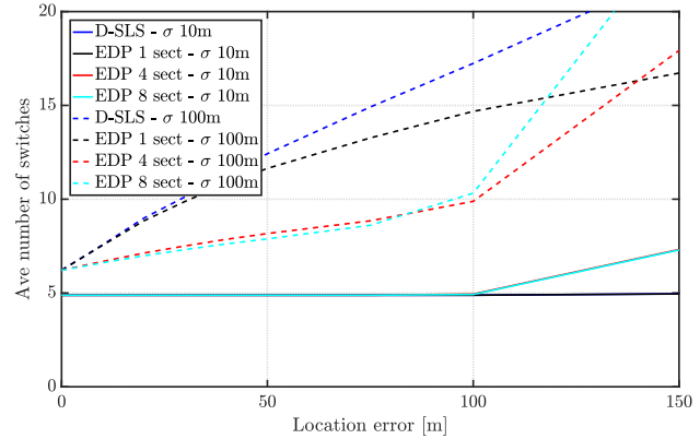
Fig. 6. Performance evaluation for different BS discovery procedures and \sigma of the user normal distribution.
