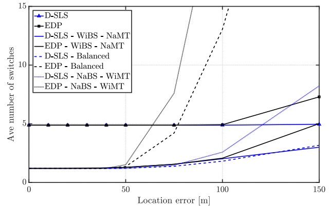
(b) Population of 1000 users normally distributed with \sigma = 10 .
