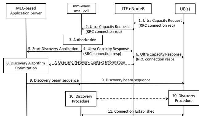
Fig. 14. Flow diagram for Cell Discovery Procedure in 3GPP architecture.
