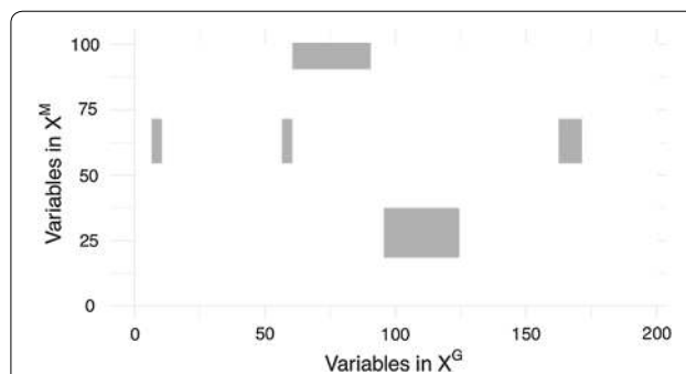
Fig. 3 Illustration of the true block interaction matrix \theta with l = 5 , \sigma = 0.5 and n = 100 . Each non-zero value in this matrix is considered as a true interaction between two variables
