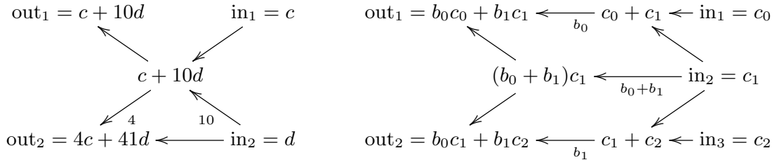
Fig. 4.2. Transposing the algorithms in Figure 4.1.
