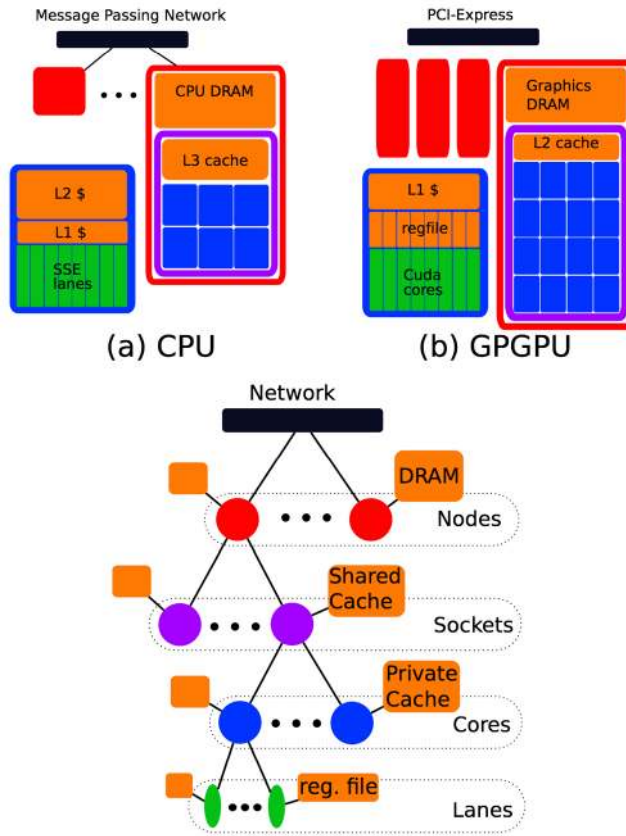
Figure 2. The four-level hierarchy of modern parallel systems. Nodes contain disjoint DRAM address spaces, and communicate over a message-passing network in the CPU case, or over a shared PCI-Express network in the GPU case. Sockets within a node (only one shown) share DRAM but have private caches – the L3 cache in CPU systems and the L2 cache in Fermi-class systems. Similarly Cores share access to the Socket-level cache, but have private caches (CPU L2, GPU L1/scratchpad). Vector-style parallelism within a core is leveraged via Lanes – SSE-style SIMD instructions on CPUs, or the SIMT-style execution of GPUs.
