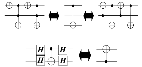
Fig. 5. Equivalent circuit templates.
