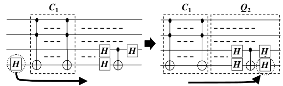
Fig. 6. Transforming a miter circuit after simplification. Dashed boxes outline circuit modules. Horizontal dashed lines represent omitted qubits and gates.
