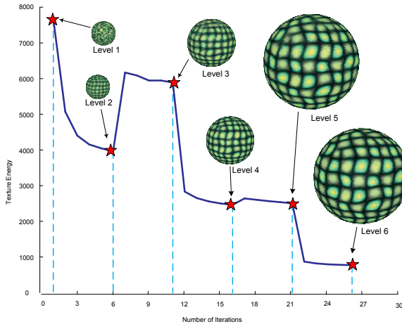
Fig. 2 Texture energy plotted as a function of number of iterations. The energy is normalized with respect to output resolutions as in [4]. Also shown is the synthesized texture after each resolution and scale (neighborhood size) level.
