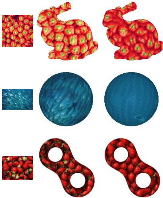
Fig. 4 Comparison of our solver with the least square one in [4]. For each group of images, the input is on the left, our result is in the middle, and the result via least square solver [4] is on the right.
