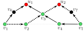
Figure 3: Landmark-BFS technique. Here, solid arrows belong to the SPT of u_1 , and dotted arrows belong to the SPT of u_2 .
