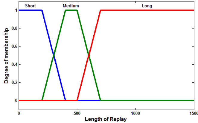
Figure 4. Membership Function of First Input: Length of Replay ( L_{Replay} )
