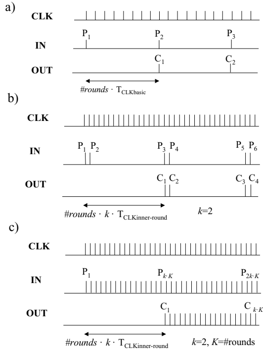
Figure 5. Input/output timing characteristics of various architectures. a) basic iterative architecture b) inner-round pipelining c) full mixed inner and outer-round pipelining
