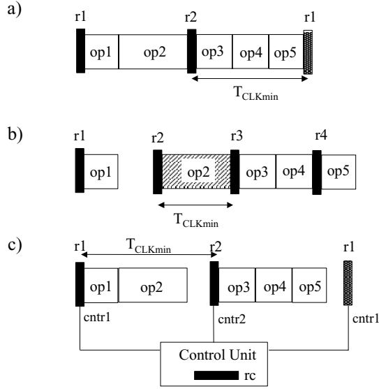
Figure 6. Limits on the minimum clock period in the architecture with inner-round pipelining. a) ideal situation; evenly divided round, b) clock period limited by the largest indivisible operation, c) clock period limited by the control unit, i.e., the time necessary to generate and distribute control signals.
