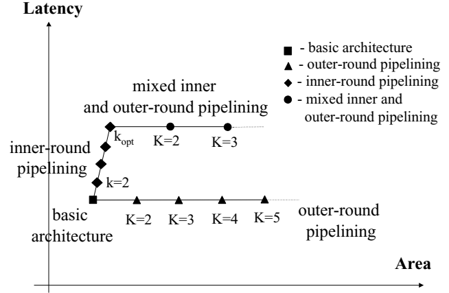
Figure 4. Impact of the inner-round and outer-round pipelining on latency.
