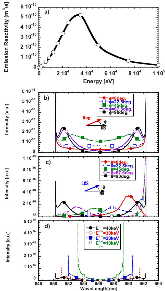
FIG. 2. (Color online) (a) Energy dependence of the charge exchange reaction rate for the hydrogen to hydrogen ( n=3 ) charge transfer process. Variations of the Doppler shifted H_{\alpha} -spectra for monoenergetic fast ions with the change in the (b) NB-injection pitch angle, (c) the angle between NB-injection path, and the LOSs, and (d) the energy of gyrating fast ions. The directions of the LOS, the magnetic field lines and the NB-injection can be considered orthogonal to one other if the angle between them is not indicated.
