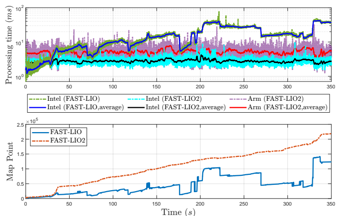
Fig. 8. The processing time for each LiDAR scan of FAST-LIO and FAST-LIO2.
