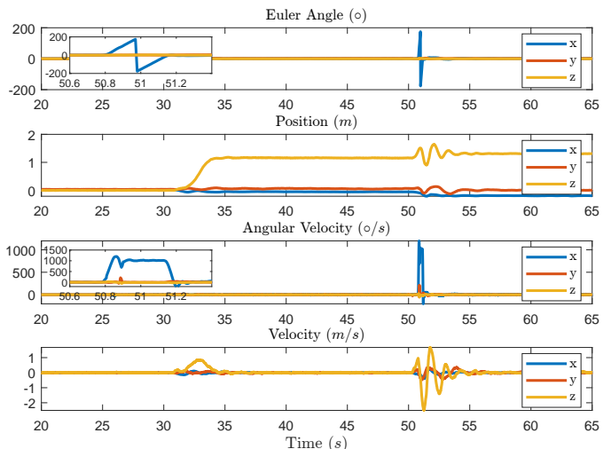
Fig. 11. The attitude, position, angular velocity and linear velocity in the UAV flip experiments.
