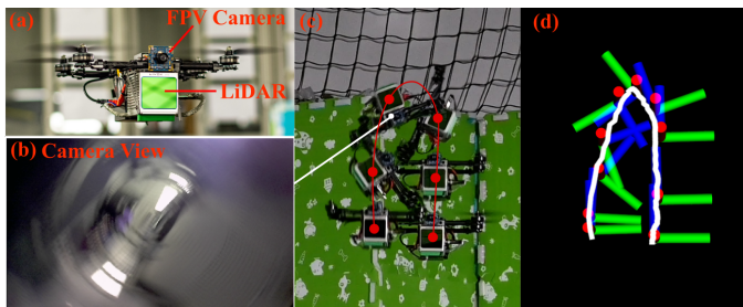
Fig. 9. The flip experiment. (a) the small scale UAV; (b) the onboard camera showing first person view (FPV) images during the flip; (c) the third person view images of the UAV during the flip; (d) the estimated UAV pose with FAST-LIO2.
