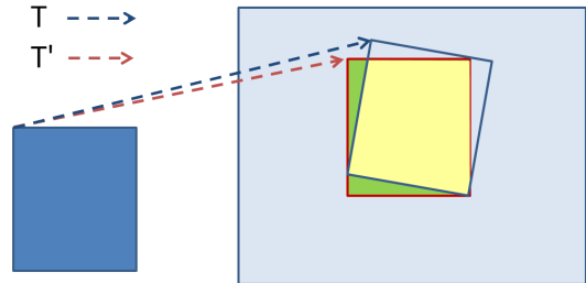
Fig. 1. A template mapped to an image by two close transformations. The close transformations map the template to close parallelograms. The error of T' cannot be very different from that of T . Most of the change in error is from different points being mapped to the intersection area (in yellow). This difference depends on the total variation of the template. The remaining error depends on the green area which is small because the transformations are close.
