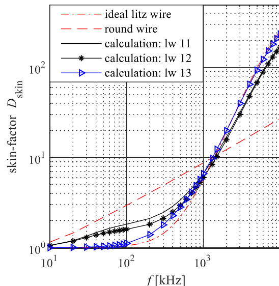
Fig. 13. Fast numerical calculation of the frequency-dependent skin factor for different twisting structures of a litz wire consisting of 1000 strands (cf. Table II). The skin factor D_{\text{skin}} is plotted for frequencies up to 10 MHz. In addition, the analytic results for a perfectly twisted (ideal) litz wire and a round conductor with the same dc resistance are visualized.
