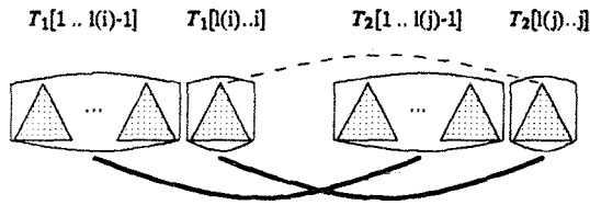
Figure 7. Case 3. holds when (i, j) is in mapping
