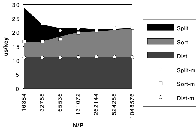
Figure 15: Estimated and measured execution times of various phase of sample sort on 512 processors.
