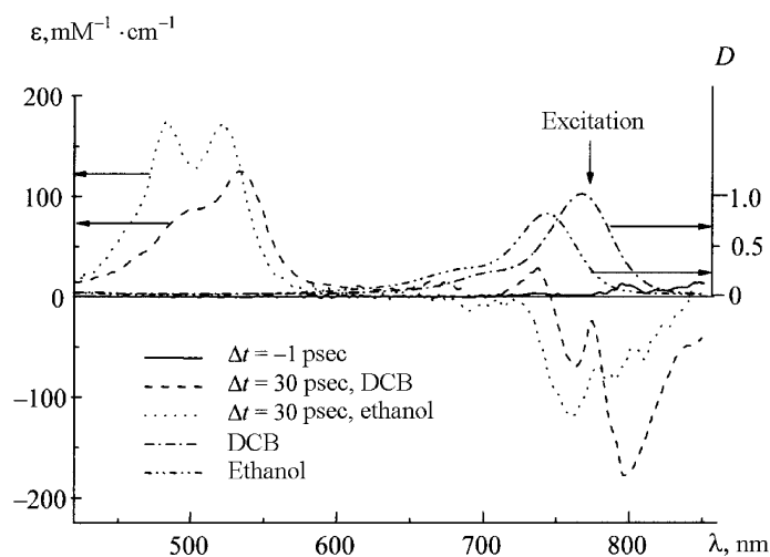
Fig. 4. Absorption spectra normalized for excitation from the excited state and stationary spectra of dye HITC solutions in dichlorobenzene and ethanol.
