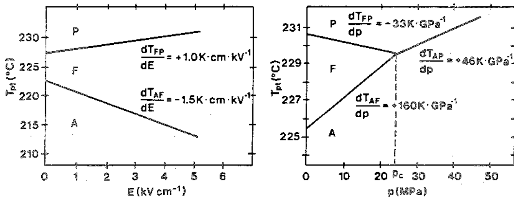
Fig. 3 The dependence of phase-transition temperatures T_{pt} on a) the applied electric field strength [2] and b) hydrostatic pressure for \text{PbZrO}_3 [2, 3].
