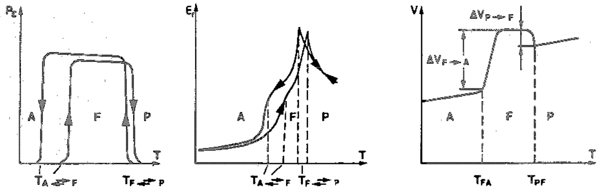
Fig. 2 The temperature dependence of a) spontaneous polarization \bar{P}_s , b) electric permittivity \epsilon_r , and c) unit cell volume V, for \text{PbZrO}_3 and \text{Pb}(\text{Zr},\text{Ti})\text{O}_3 with A-F-P phase-transition sequences [4, 5].
