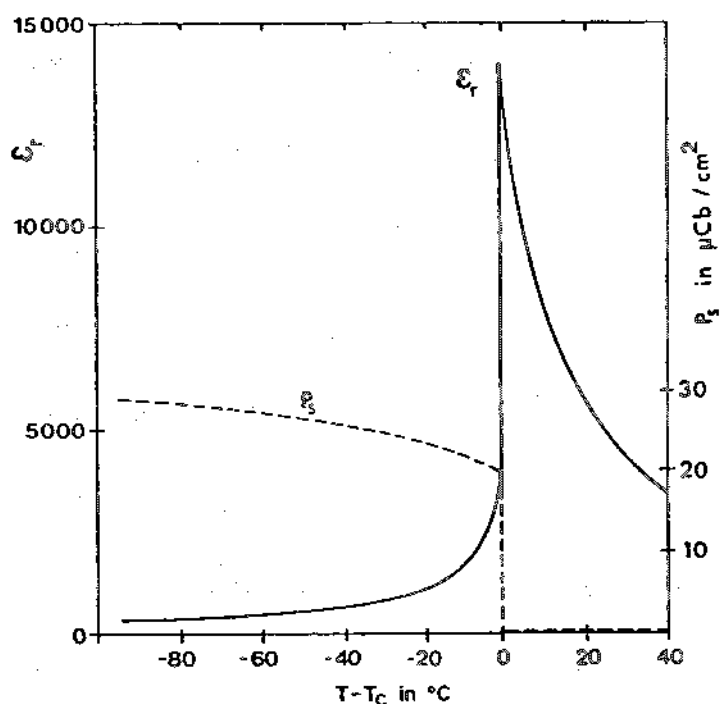
Fig. 1 Temperature dependence of spontaneous polarization \vec{P}_s and dielectric constant \epsilon_r near the Curie point T_c , in the case of a first-order phase transition (example: \text{BaTiO}_3 single crystal).
