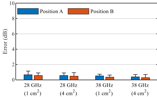
Fig. 15. The mean and maximum values of the reconstruction errors for the 1\text{ cm}^2 and 4\text{ cm}^2 psaPD at 28 GHz and the 1\text{ cm}^2 and 4\text{ cm}^2 psaPD at 38 GHz reconstructed from the simulated IF data when the origin is set at different positions. Each bar contains 124 samples from different combinations of antenna (Ant 1–4) and evaluation distance (from d = 5\text{ mm} to d = 35\text{ mm} with 1\text{ mm} step).
