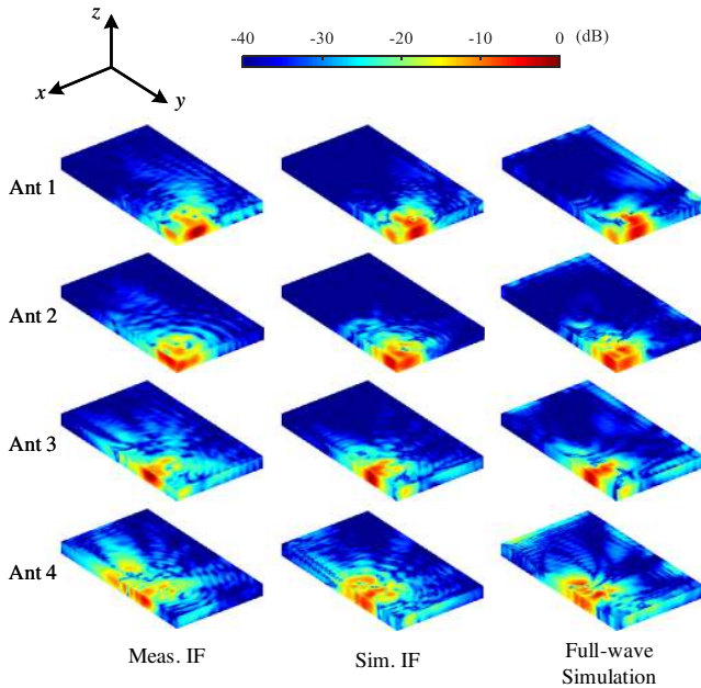
Fig. 5. The PD distributions at 28 GHz reconstructed from measured IF (left column), reconstructed from simulated IF (middle column) and computed from full-wave simulation (right column) on the outer surface of a closed box embracing the DUT from the outside with a 5 mm gap. The PD distributions are normalized with 20 \text{ W/m}^2 .
