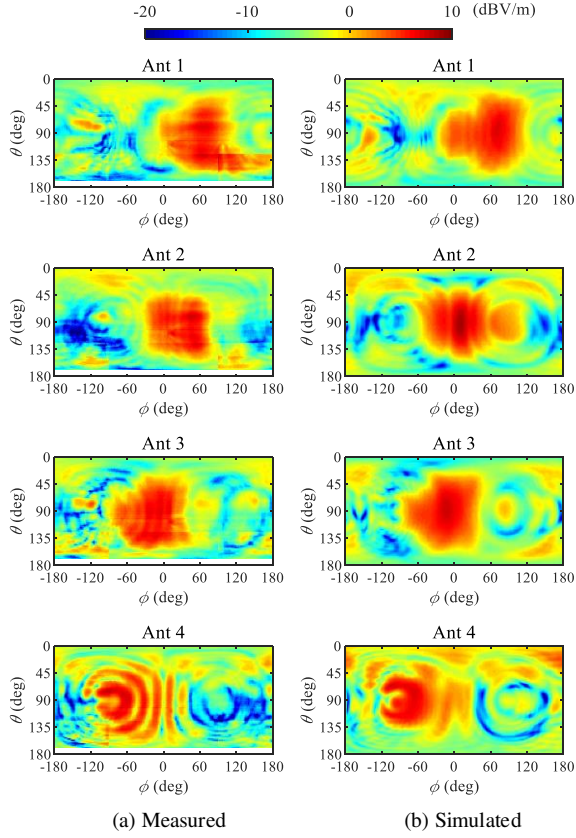
Fig. 3. (a) The measured and (b) simulated |\mathbf{E}| distributions over \Sigma_M , a sphere with radius of 450 mm, in the IF region of Ant 1–Ant 4 at 28 GHz. The input power is normalized to 5 dBm.
