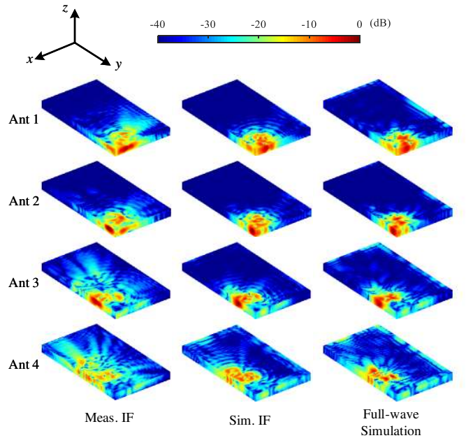
Fig. 6. The PD distributions at 38 GHz reconstructed from measured IF (left column), reconstructed from simulated IF (middle column) and computed from full-wave simulation (right column) on the outer surface of a closed box embracing the DUT from the outside with a 5 mm gap. The PD distributions are normalized with 20 \text{ W/m}^2 .
