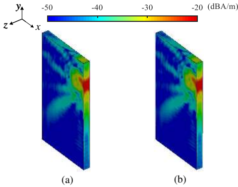
Fig. 14. |J_{eq}| distributions reconstructed from the simulated IF data of Ant 3 at 28 GHz when the origin is set at (a) Position A and (b) Position B.
