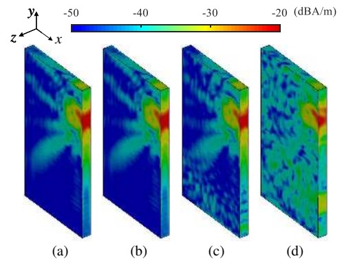
Fig. 9. |J_{\text{eq}}| distributions reconstructed from the simulated IF data of Ant 3 at 28 GHz with the angular resolution of (a) \Delta\alpha = 2^\circ , (b) \Delta\alpha = 4^\circ , (c) \Delta\alpha = 6^\circ , and (d) \Delta\alpha = 8^\circ .
