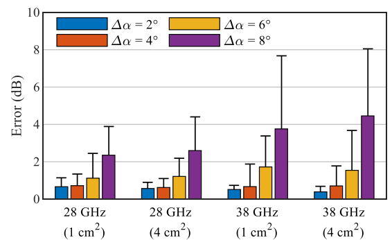
Fig. 10. The mean and maximum values of the reconstruction errors for the 1 \text{ cm}^2 and 4 \text{ cm}^2 psaPD at 28 GHz and the 1 \text{ cm}^2 and 4 \text{ cm}^2 psaPD at 38 GHz reconstructed from the simulated IF data with different values of angular resolution \Delta\alpha . Each bar contains 124 samples from different combinations of antenna (Ant 1–4) and evaluation distance (from d = 5 mm to d = 35 mm with 1 mm step).
