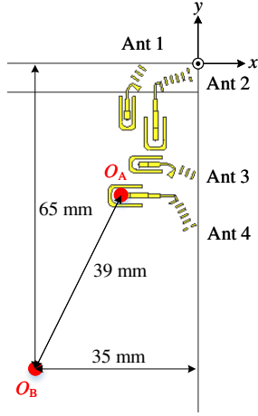
Fig. 13. For Ant 4 under test, the origin of the spherical coordinate system can be set at Position A ( O_A ) or Position B ( O_B ).
