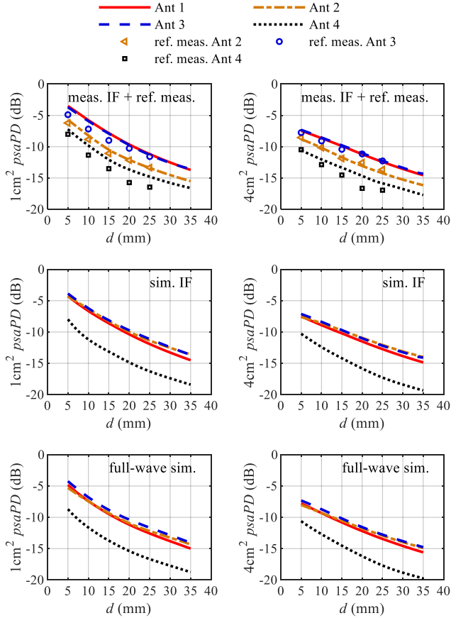
Fig. 7. The 1 \text{ cm}^2 (left column) and 4 \text{ cm}^2 (right column) psdPD at 28 GHz as the evaluation distance varies for Ant 1–Ant 4. The values are normalized with 20 \text{ W/m}^2 .
