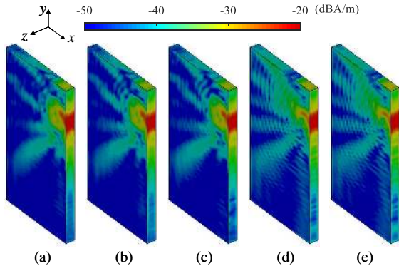
Fig. 11. |J_{\text{eq}}| distributions reconstructed from the simulated IF data of Ant 3 at 28 GHz with the phase noise level of (a) \sigma = 0^\circ , (b) \sigma = 5^\circ , (c) \sigma = 10^\circ , (d) \sigma = 15^\circ , and (e) \sigma = 20^\circ .
