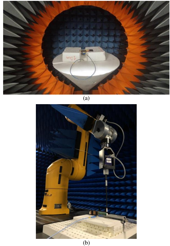
Fig. 2. (a) The measured IF data is collected by MVG StarLab 50 GHz and (b) the NF is measured by SPEAG cDASY6 mmWave Module V1.0 and EUmmWV3 probe.
