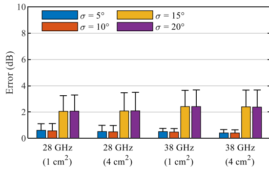
Fig. 12. The mean value and the 95 % confidence range of the reconstruction errors for the 1 cm 2 and 4 cm 2 psaPD at 28 GHz and the 1 cm 2 and 4 cm 2 psaPD at 38 GHz reconstructed from the simulated IF data with different levels of noise. Each bar contains 620 samples from different combinations of \phi_n distribution (five distributions at each noise level), antenna (Ant 1–4), and evaluation distance (from d = 5 mm to d = 35 mm with 1 mm step).
