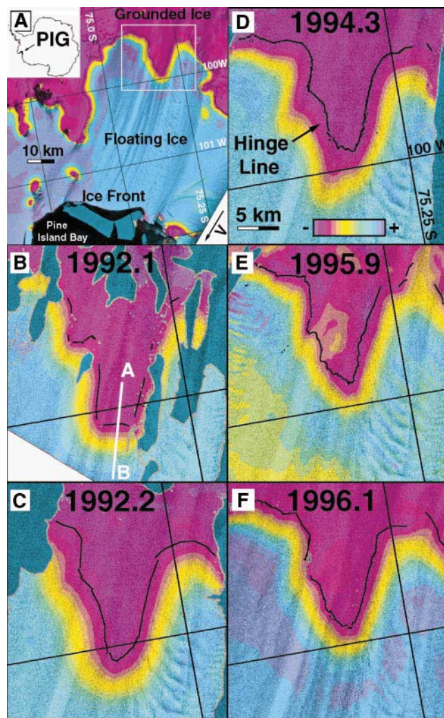
Fig. 1. Normalized tidal displacements of Pine Island Glacier (PIG), West Antarctica, recorded with ERS differential interferometry and color coded [color bar in (D)] from magenta (grounded ice) to yellow (glacier flexure zone) and blue (ice-shelf ice in hydrostatic equilibrium with the ocean waters). Color tone is modulated by the radar brightness of the scene acquired by ERS-1 on 21 January 1996 (orbit 23,627, frames 5589 and 5607). The glacier fast moving portion is revealed by flow-line features conspicuous in the radar brightness image. No interferometric data are available in areas colored dark green. The white square in (A) delineates the area shown in (B) to (F). ERS is flying north in (A), (B), and (F) (ascending track, heading -49° from N) and south in (C), (D), and (E) (descending track, heading -128° from N), illuminating the scene from its right. The tide normalization factors from (B) to (F) are 2.2, 4.0, 3.2, 2.7, and 0.9 m, respectively. The hinge-line position, retrieved from model fitting (14), is shown as a black, thin, continuous line separating grounded (magenta, minus sign) from floating ice (blue, positive sign). Its finger-shaped appearance in (B) to (F) indicates the presence of thicker ice at the glacier center than along its sides. In (A), locally grounded areas or ice rises appear in magenta between the hinge line and the ice front, in areas where the ice shelf is virtually stagnant. Profile A-B [thick, white line in (B)] is discussed in Fig. 2A. Hinge-line position and tidal displacements were recorded in (B) January 1992 (ERS-1 orbits 2970, 3056, and 3142; frame 5589), (C) February 1992 (ERS-1 orbits 3260, 3346, and 3432; frame 5211), (D) March 1994 (ERS-1 orbits 13,826, 13,869, and 13,912; frame 5211), (E) November 1995 and January 1996 (ERS-1/2 orbit pairs 22,614/2941 and 23,616/3943; frame 5211), and (F) January and February 1996 (ERS-1/2 orbit pairs 23,627/3954 and 24,128/4455; frame 5589). Between (B) and (F), the hinge line retreated 5.0 ± 1.0 km in 3.78 years over a 275-m-wide region at the glacier center. The retreat is less along the side margins presumably because of steeper slopes (-1.2% instead of -0.5% at the glacier center) and possibly less thinning (21).
