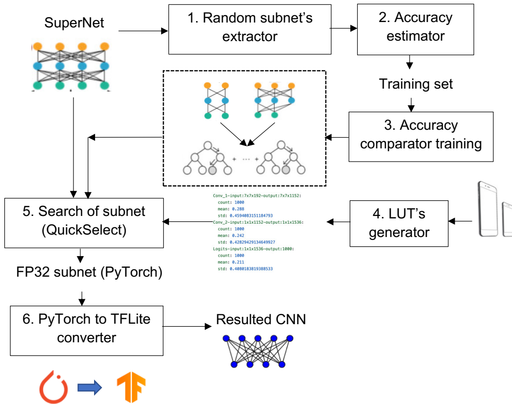
FIGURE 1: The proposed approach for fast adaptation of face recognition models.
