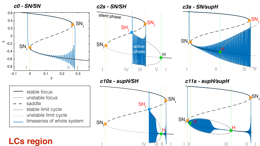
Fig. 6 Bifurcation diagrams along bursting paths. For each bursting class found in the unfolding we produced the bifurcation diagram of the fast subsystem using z as bifurcation parameter and plotting the fast variable x as ordinate. The simulated bursting trajectory, in blue, is superimposed to the bifurcation diagram. Bifurcations are marked with a colored star (same color code as in Fig. 4) and vertical dotted line of the same color separate regions of the unfolding. The Roman numeral of the relative region is written in gray in the lower part of the plots. Onset and offset bifurcations are written in red. In all the nine classes (eight point-cycle and one point-point bursters) the upper branch of the z-shaped curve of fixed points acts as silent state. When the fast subsystem is in the silent state, the slow variable z is instructed to increase. At SN_r (or at the subcritical Hopf point in classes c14b and c16b) the resting-state destabilizes, the system moves towards another attractor, and z start decreasing until the system goes back to the silent state and a new bursting cycle is started. The active phase takes place on the limit cycle surrounding the lower branch of the equilibrium manifold. The top panel shows bifurcation diagrams for bursters in the LCs region, the bottom panel for those in the LCb region. In the LCs region we can have a saddle-node onset if the limit cycle exists already when the silent state destabilizes at SN_r (first row) or supercritical Hopf onset when the limit cycle is created for smaller values of z (second row). Oscillations can end because the limit cycle coalesces with the saddle (middle column) or because of another supercritical Hopf bifurcation (right column). In the LCb region panel, in the first row oscillations are started through saddle-node bifurcation, while the resting-state destabilizes earlier in the second row via subcritical Hopf bifurcation. The limit cycle coalesces with the saddle in the left column and with an unstable limit cycle in the right column. Bursting paths and entire arcs of great circles used to produce these bifurcation diagrams are shown in Sect. 5.3
