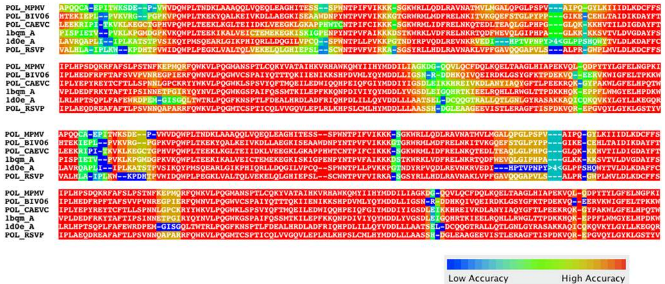
Figure 5. The Java GUI allows users to visualize the estimated alignment accuracy under FSA's statistical model. FSA's alignment is colored according to the expected accuracy under FSA's statistical model (top) as well as according to the "true" accuracy (bottom) given from a comparison between FSA's alignment and the reference structural alignment. It is clear from inspection that accuracies estimated under FSA's statistical model correspond closely to the true accuracies. Sequences are from alignment BBS12030 in the RV12 dataset of BALIBASE 3 [24]. doi:10.1371/journal.pcbi.1000392.g005
