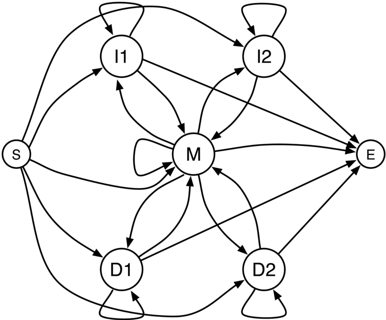
Figure 2. The default Pair HMM used by FSA. By default FSA uses a Pair HMM with two sets of Insert (I) and Delete (D) states to generate a two-component geometric mixture distribution. FSA can optionally use a three-state HMM, which has only one set of Insert and Delete states. M is a Match state emitting aligned characters. doi:10.1371/journal.pcbi.1000392.g002
