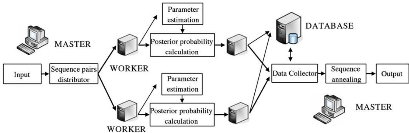
Figure 4. Schematic overview of FSA's parallelization strategy on a computer cluster. For large input sizes, a disk-based database may be used to store some of the primary data structures and reduce memory usage. doi:10.1371/journal.pcbi.1000392.g004
