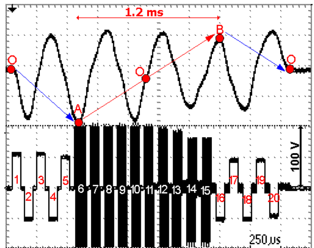
Fig.7. Fast optical retardation switching with \Delta L = 10 \Delta L \approx 1.6 \mu\text{m} in \tau_{A \rightarrow B} \approx 1.2\text{ms} , where A and B are states of the dual frequency liquid crystal in Fig.8.
