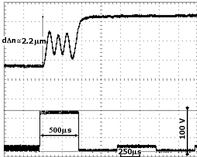
Fig.5. Fast optical retardation shift on \Delta L \approx 2.2 \mu\text{m} by one SSP.
