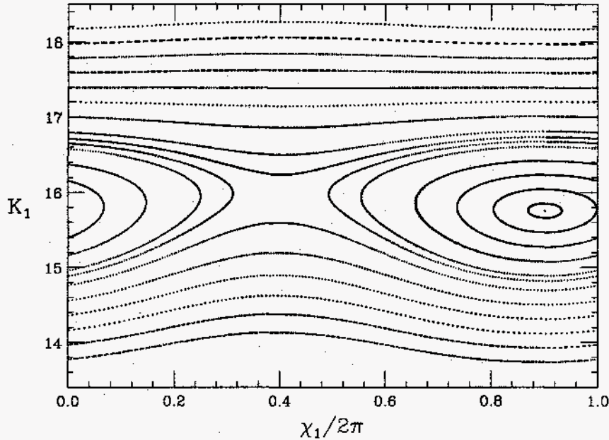
FIGURE 8. A plot of K_1 vs. \chi_1 \pmod{2\pi} for several orbits in the [6,1] resonance region. All orbits have the same initial value of K_2 . Units: 10^{-8}m .
