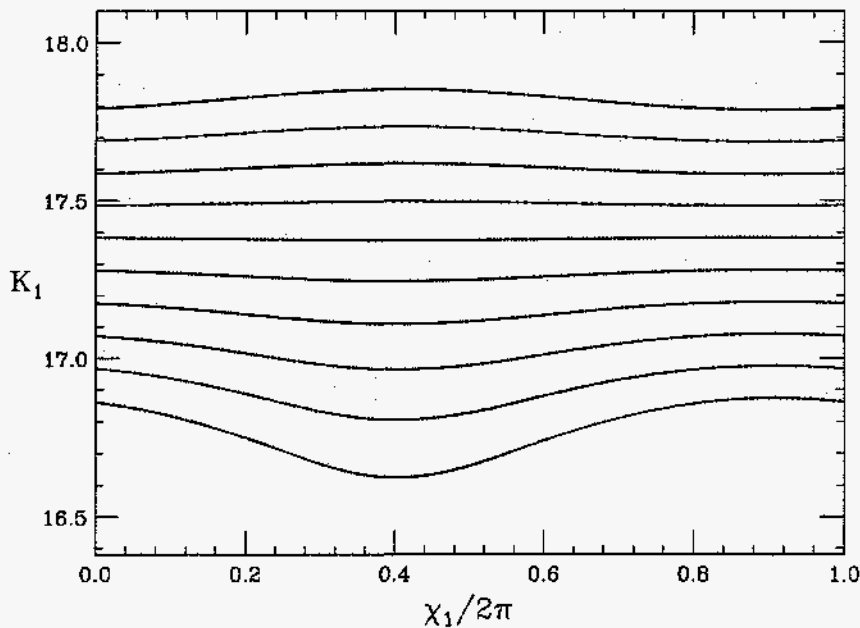
FIGURE 15. Data for 10 rotational pendulum orbits and the curves obtained by fitting them to Fourier series with 8 modes. The orbits all have the same initial value of K_2 . The data are barely distinguishable from the curves at the resolution of the plotter.
