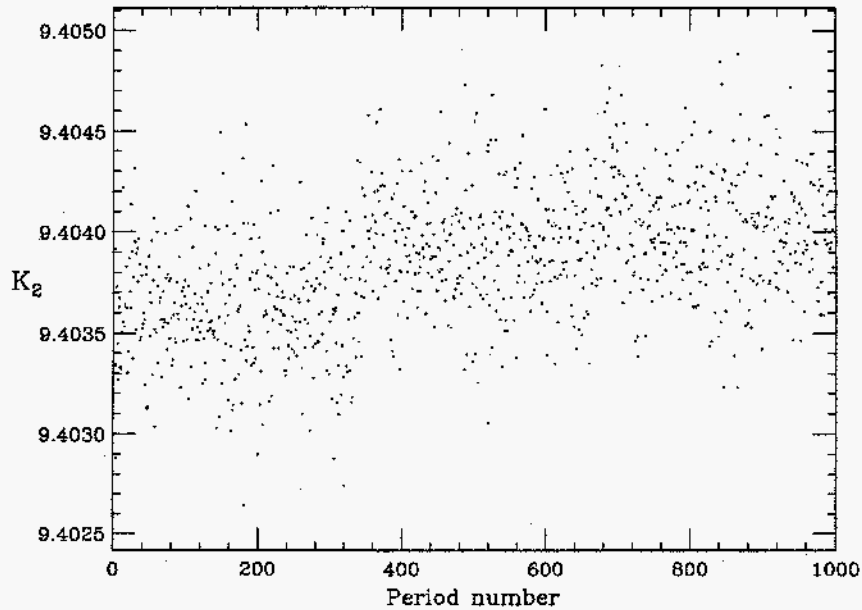
FIGURE 9. A plot showing fluctuations of K_2 along a single orbit in the [6,1] resonance region. Units: 10^{-8}m .
