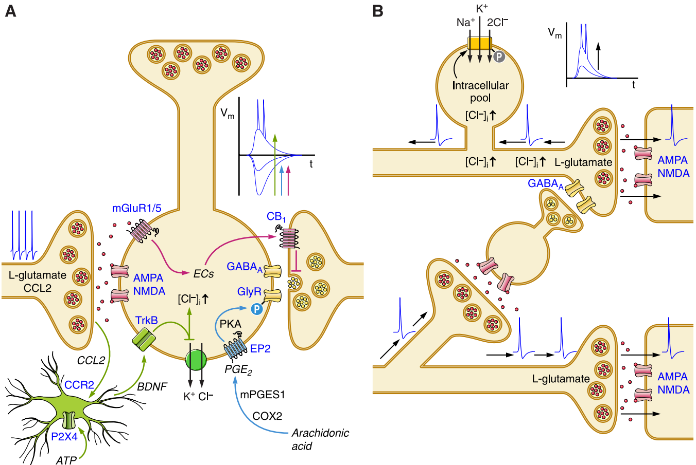
FIGURE 15 Possible changes in synaptic inhibition during pathological pain states. A : three pathways leading to reduced synaptic inhibition in the dorsal horn. Peripheral nerve damage and microglia-induced changes in the inhibitory control by GABA and glycine (pathway shown in green). Inflammation-induced reduction in glycinergic neurotransmission (blue). Reduced glycine and GABA release triggered by intense C fiber input and subsequent release of endocannabinoids and activation of presynaptic CB 1 receptors (magenta). B : dorsal root reflexes as a possible source of secondary hyperalgesia and allodynia. Input from the lower axon excites a GABAergic interneuron, which depolarizes the top axon terminal. If the intracellular chloride concentration of the top axon is sufficiently high and input from the GABAergic interneuron strong enough to reach the action potential threshold, the top axon would give rise to the activation of additional central neurons and to release of proinflammatory peptides through action potentials retrogradely invading the periphery.
