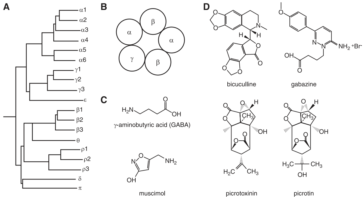
FIGURE 3 GABA A receptor subunits and ligands. A : dendrogram of mammalian GABA A receptors. [Modified from Barnard (30).] B : wheel arrangement of the five subunits of a typical GABA A receptor containing \alpha , \beta , and \gamma subunits seen from the extracellular side. [Data based on Baumann et al. (32, 33).] C : chemical structures of GABA and of the GABA A receptor agonist muscimol. D : chemical structures of GABA A receptor blockers.
