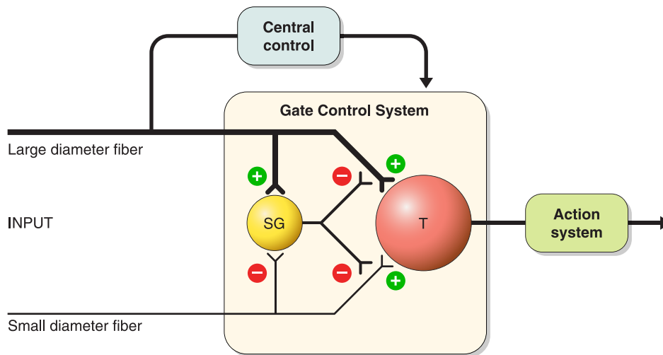
FIGURE 1 Gate control theory of pain. This model proposed that inhibitory interneurons (yellow) located in the substantia gelatinosa (SG) would determine whether nociceptive input from the periphery would be relayed through the spinal transmission system (red, T) to higher CNS areas where pain would be consciously perceived. [Modified from Melzack and Wall (248), with permission from AAAS.]
