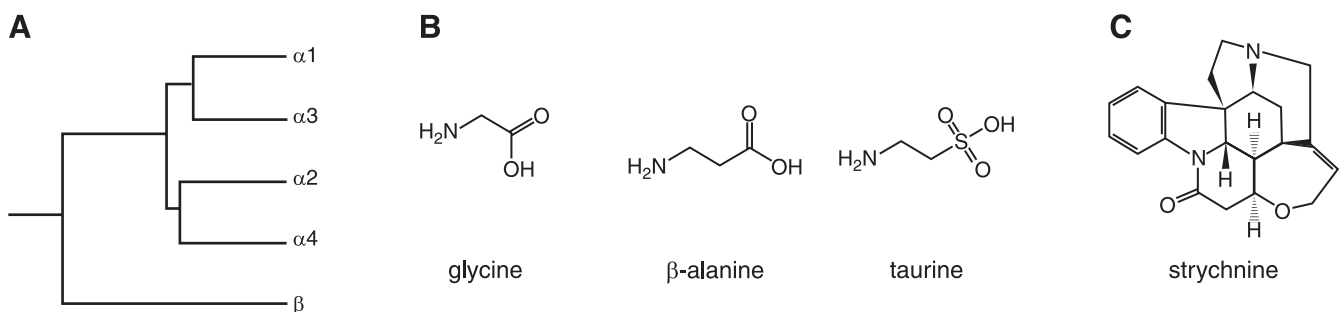
FIGURE 4 Inhibitory (strychnine-sensitive) glycine receptor subunits and ligands. A : dendrogram of mammalian inhibitory glycine receptors. B : chemical structures of glycine and of other putative endogenous glycine receptor agonists \beta -alanine and taurine. C : chemical structure of the glycine receptor antagonist strychnine.
