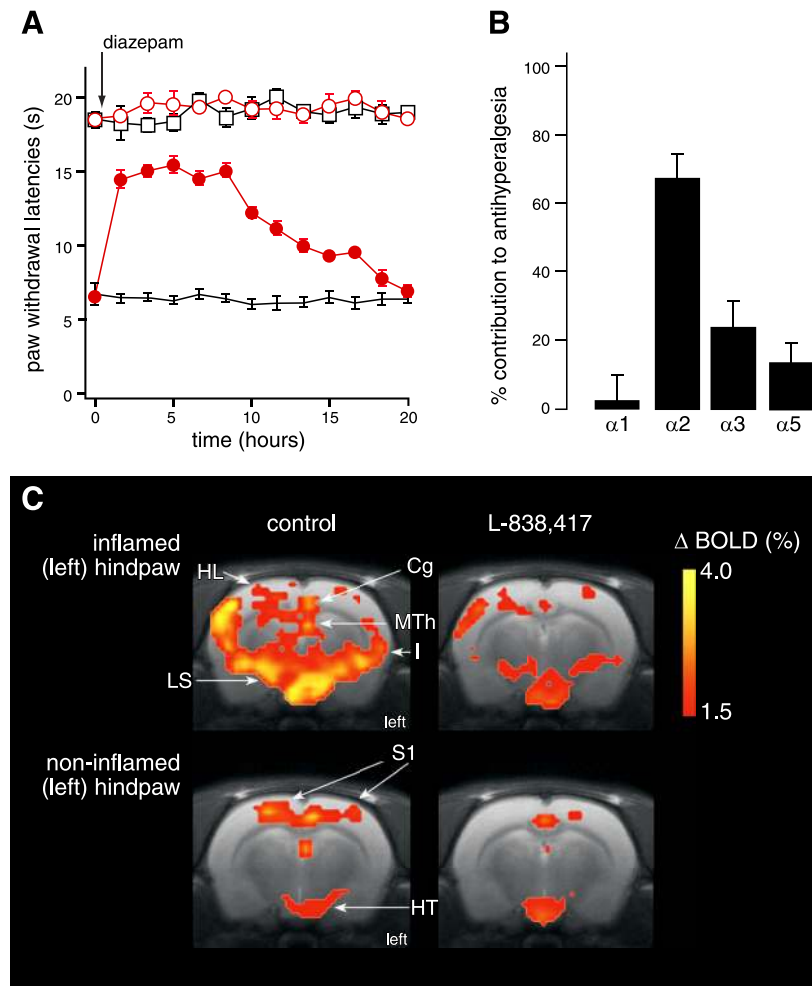
FIGURE 16 Antihyperalgesic actions of spinally injected diazepam and the contribution of the different GABA A receptor subtypes. A : antihyperalgesic action of intrathecal injection of diazepam (0.09 mg/kg, red symbols; vehicle, black) in mice with inflammatory hyperalgesia induced by subcutaneous injection of zymosan A. Open symbols represent contralateral noninflamed paw. Note the lack of effect on the contralateral noninflamed paw. B : contribution of the different diazepam-sensitive GABA A receptor subtypes to antihyperalgesia against inflammatory pain. C : antihyperalgesic activity of systemically administered L-838,417, a subtype selective ( \alpha 1-sparing) GABA A receptor modulator visualized in a rat functional magnetic resonance imaging (fMRI) experiment. Inflamed and noninflamed (contralateral) hindpaws were stimulated with a defined heat stimulus, and brain activation was measured. Note again the pronounced reduction in brain activation after stimulation of the inflamed paw, and the considerably smaller effect on activation following stimulation of the noninflamed paw. [Modified from Knabl et al. (196).]
