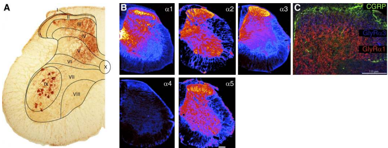
FIGURE 6 Laminal organization of the spinal cord and distribution of inhibitory neurotransmitter receptors. A: spinal laminae illustrated in a coronal section of the lumbar spinal cord taken from a mouse whose sciatic nerve has been injected with cholera toxin B subunit to label axons and terminals of myelinated sensory nerve fibers and motoneurons. [Courtesy of Drs. Jolly Paul and Jean-Marc Fritschy.] B: distribution of GABA A receptor subunits is shown as pseudocolor images. Highest density, yellow; low density, blue. [Modified from Zeilhofer et al. (417).] C: distribution of glycine receptor subunits GlyR \alpha 1 and GlyR \alpha 3 in the spinal dorsal horn. Counterstaining is against calcitonin gene-related peptide, which marks lamina II outer. [Modified from Harvey et al. (140)., with permission from AAAS.]
