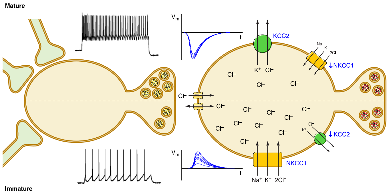
FIGURE 12 Possible “deficits” in inhibitory synaptic control in the immature GABAergic neuron. Top and bottom parts of the figure depict proposed characteristics of the mature and immature synaptic inhibition, respectively. Weaker excitatory drive onto inhibitory interneurons, higher intracellular chloride concentration, lower chloride extrusion capacity, lower membrane excitability, and less reliable transmitter release have been proposed for the immature GABAergic neuron.
