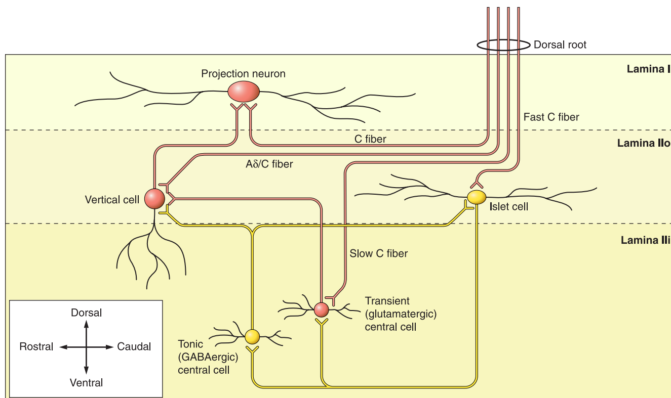
FIGURE 10 Synaptic connections in the superficial dorsal horn. Excitatory and inhibitory neurons are depicted in red or yellow, respectively. [Diagram based on data from the groups of Perl (226, 227, 422) and Yoshimura (406).]
