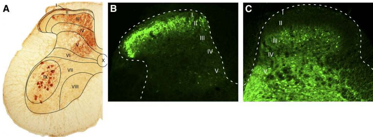
FIGURE 7 Distribution of GABAergic and glycinergic neurons in the dorsal horn. A : dorsal horn laminae. B : distribution of GABAergic neurons visualized as EGFP expression driven by the GAD67 promoter. C : distribution of glycinergic neurons visualized through EGFP expression driven by the GlyT2 promoter.
