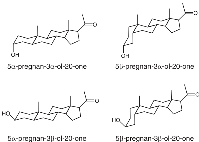
FIGURE 14 Chemical structures of neurosteroids active at GABA A receptors.
