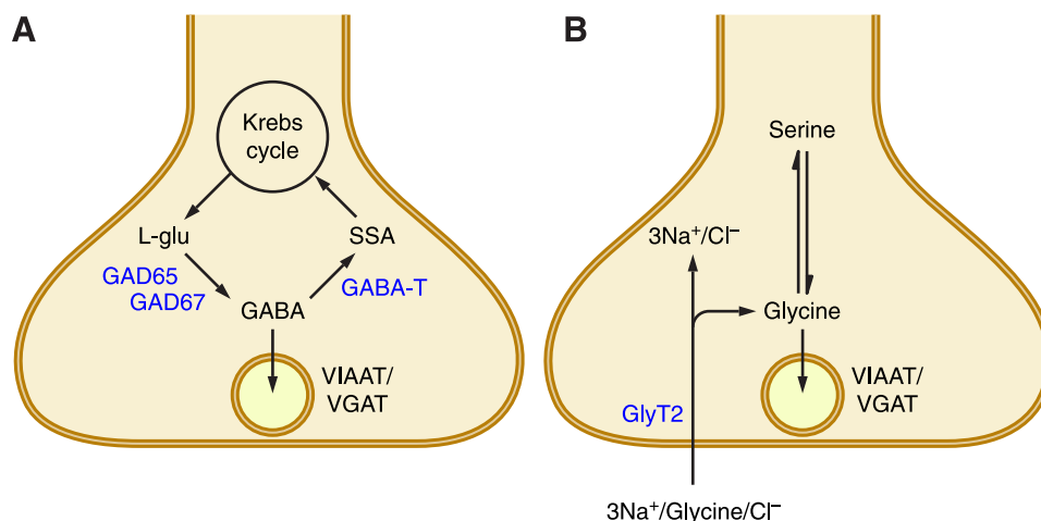
FIGURE 5 Key elements of GABAergic (A) and glycinergic (B) presynaptic terminals. GABA-T, GABA transaminase; SSA, succinyl semialdehyde.
