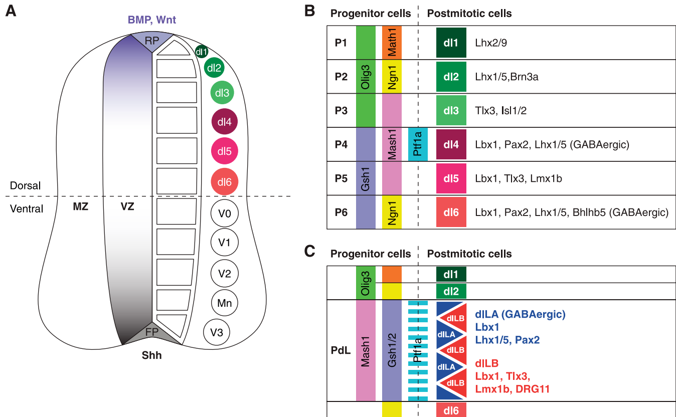
FIGURE 9 Generation of spinal interneuron diversity. A: the neural tube is patterned by morphogen gradients secreted from the floor and the roof plate (FP and RP, respectively). Morphogen activity, such as sonic hedgehog (Shh) activity from the FP or Wnt and bone morphogenic protein (BMP) activity from the RP, leads to the concentration-dependent activation or repression of various transcription factors, and thereby to the generation of distinct progenitor domains. Within the ventricular zone (VZ) of the ventral neural tube, five distinct progenitor domains are formed. Neurons that arise from the VZ populate the mantle zone (MZ). Each progenitor domain gives rise to a different type of ventral neuron. Therefore, five types of neurons are generated in the ventral spinal cord (V3, Mn, V2, V1, and V0). In the dorsal spinal cord, six types of interneurons (dl1–6) are generated from six different progenitor domains. Only the three dorsal-most populations (dl1–3) are dependent on morphogen signals from the RP, like BMPs or Wnts. The three ventral-most interneuron populations (dl4–dl6) are also generated in the absence of a dorsal signaling center. B and C: a transcription factor code for dorsal spinal interneuron specification. B: during the early phase of neurogenesis, six types of dorsal interneurons (dl1–6) arise from six distinct progenitor domains (P1–6). Individual progenitor domains (P1–P6) express a unique combination of transcription factors thereby establishing the identity of the respective interneuron population. Newborn dorsal interneurons also express a unique set of transcription factors required for the further specification of their identity. C: during the late phase of neurogenesis, mainly two types of late born interneurons (dILA and dILB) arise from a broad progenitor domain (PdL) expressing a seemingly uniform transcription factor code (e.g., Mash1 and Gsh1/2). This suggests the involvement of additional mechanisms than combinatorial expression of transcription factors to generate neuronal diversity. The two late born neuron populations are distinguished by the expression of a different set of transcription factors subsequently determining their identity.
