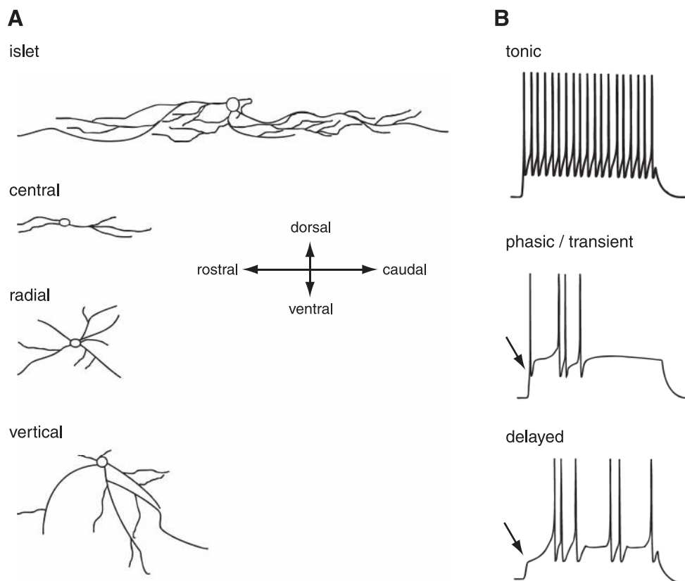
FIGURE 8 Subtypes of dorsal horn interneurons defined by the morphology of their dendritic trees ( A ) and their firing patterns ( B ). An islet cell-like morphology and tonic action potential firing are good predictors of an inhibitory (GABAergic or glycinergic) phenotype.
