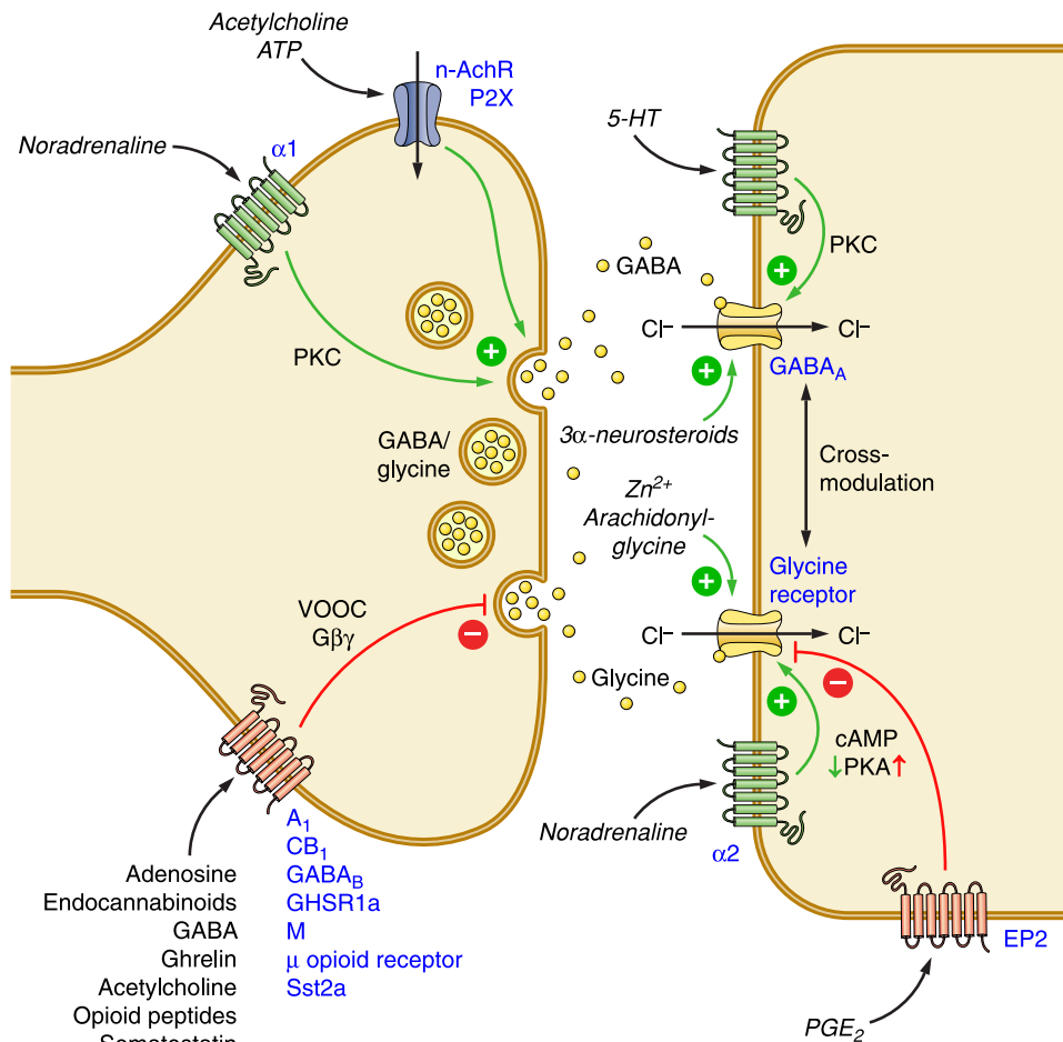
FIGURE 13 Endogenous pre- and postsynaptic modulators of inhibitory synaptic transmission in the dorsal horn.
