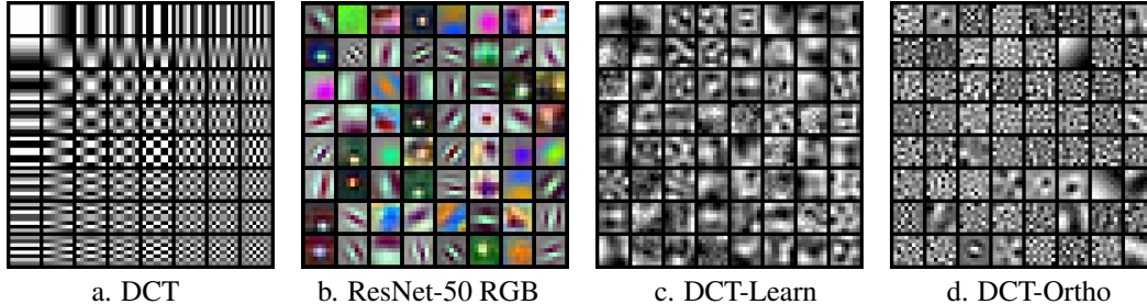
Figure 2: (a) The 64 orthonormal DCT basis vectors used for decomposing single-channel 8 \times 8 pixel blocks in the JPEG standard [26]. (b) The 64 first-layer convolution filters of size 7 \times 7 learned by a baseline ResNet-50 network operating on RGB pixels [10]. (c) The 64 convolution filters of size 8 \times 8 learned starting from random weights by the DCT-Learn network described in Sec. 4.3. (d) The 64 convolution filters from the DCT-Ortho network, similar to (c) but with an added orthonormal regularization.
