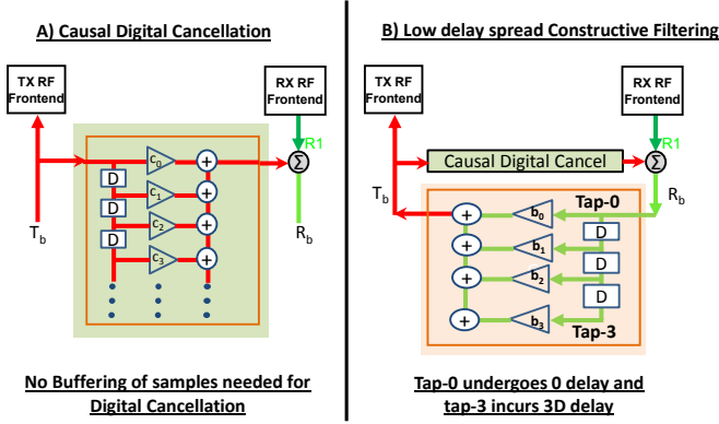
Figure 9: a) Digital cancellation in FF is causal, i.e. the cancellation is performed only using the current and past transmitted samples. No buffering of received samples is performed, which minimizes processing delay through the relay. b) The larger the number of tap delay, higher is the probability that it would cause inter-symbol interference at the destination.
