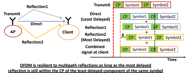
Figure 4: OFDM is resilient to multipath reflections as long as the extra delay experienced by the slowest reflection compared to the quickest arriving signal at the destination is less than the cyclic prefix (CP).
