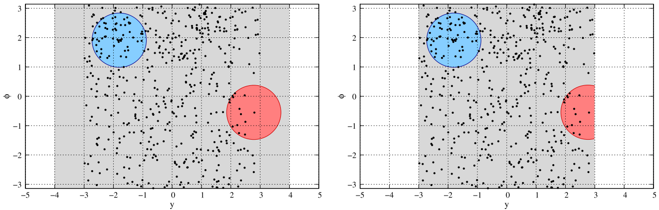
Fig. 1 Two choices for ghost placement. The grey area in each plot indicates the region containing ghosts, while the dots are particles, which here are accepted up to |y| < 3 . The circular regions indicate the areas that will be found for two particular jets. In the left-hand case, with ghosts that extend well beyond the acceptance for particles, jet areas are unaffected by the particle acceptance; in the right-hand case, with ghosts placed only up to the acceptance limit, jet areas are clipped at the edge of the acceptance
