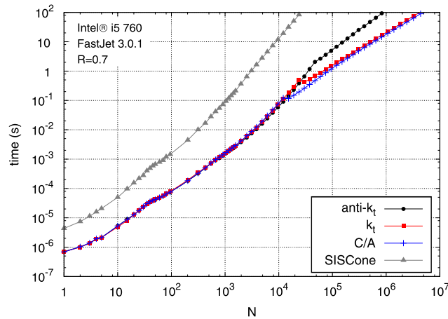
Fig. 2 Time required to perform the clustering of N particles in FastJet 3.0.1 with the Best strategy. The anti- k_t , k_t , and Cambridge/Aachen (C/A) native algorithms are shown, together with the SIS Cone plugin. All use R = 0.7 . Shown for an Intel i5 760 processor with 8 MB of cache. For small N , N was varied by taking a single hard dijet event generated with Pythia 6 [54] and extracting the N hardest particles. Large N values were obtained by taking a single hard dijet event and adding simulated minimum-bias events to it. The results include the time to extract the inclusive jets with p_t > 5 GeV and sort them into decreasing p_t
