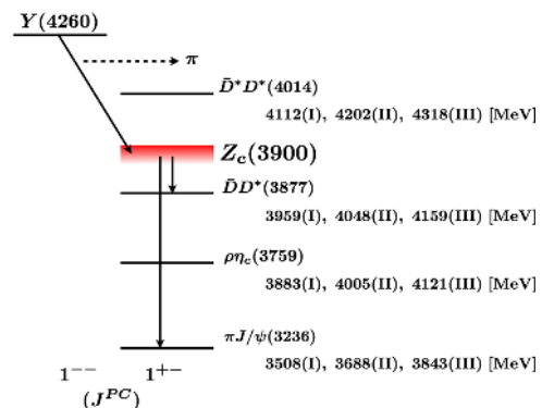
FIG. 1. A possible decay scheme of the Y(4260) through Z_c(3900) , together with the relevant two-meson thresholds of the Z_c(3900) decay at m_\pi \approx 140 (Expt.), 410 (case I), 570 (case II), and 700 (case III) MeV. The arrows represent the observed decay modes in the experiments [2–4].
