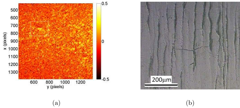
Figure 15: (a) Displacement field expressed in pixel measured by using Q4-DIC (element size: 4 \times 4 pixels) for N_c = 300,000 cycles (1 pixel \leftrightarrow 3.2 \mu\text{m} ). (b) Replica observation performed after N_c = 300,000 cycles.
