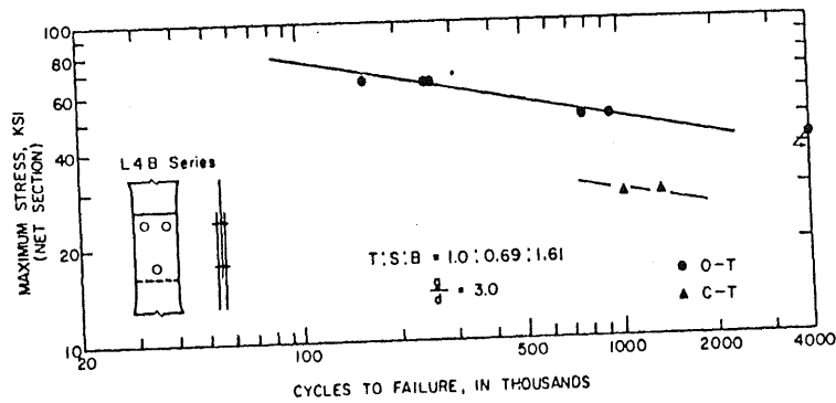
FIG. 4.—FATIGUE TESTS ON A440 STEEL IN CONNECTIONS USING A490 BOLTS (NET SECTION STRESSES)
