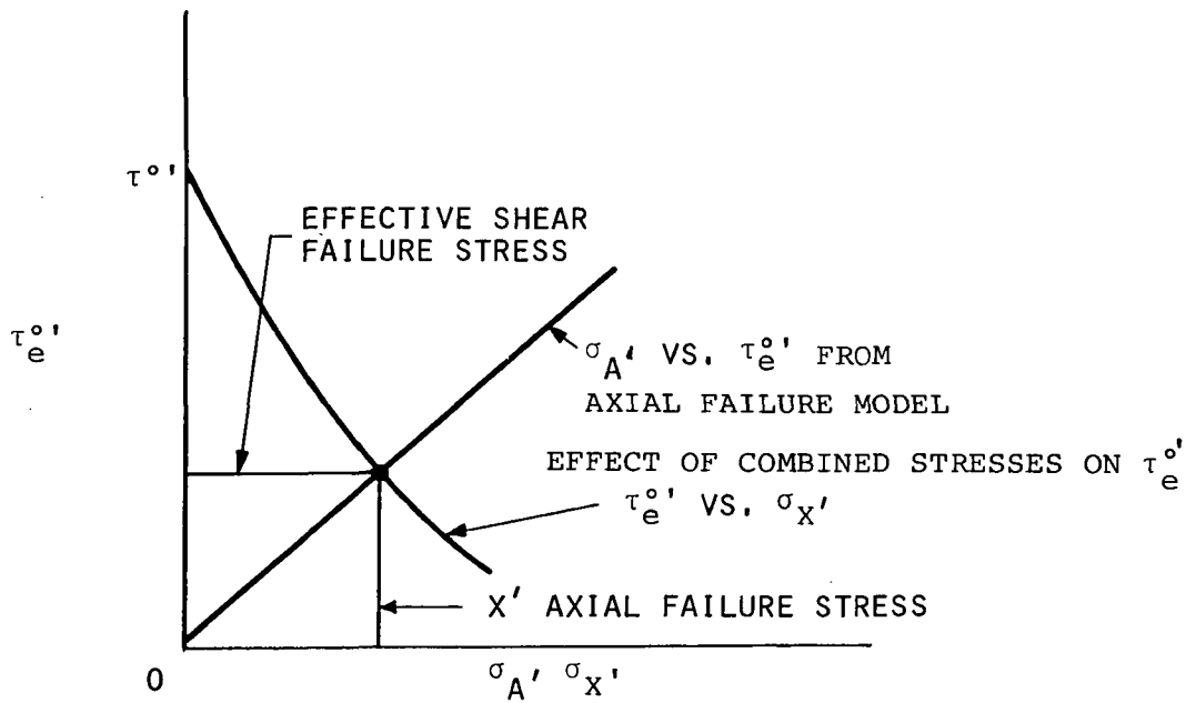
FIGURE 8. GRAPHICAL PROCEDURE FOR DETERMINING OFF-AXIS RESIDUAL STRENGTH OF NOTCHED LAMINATE
