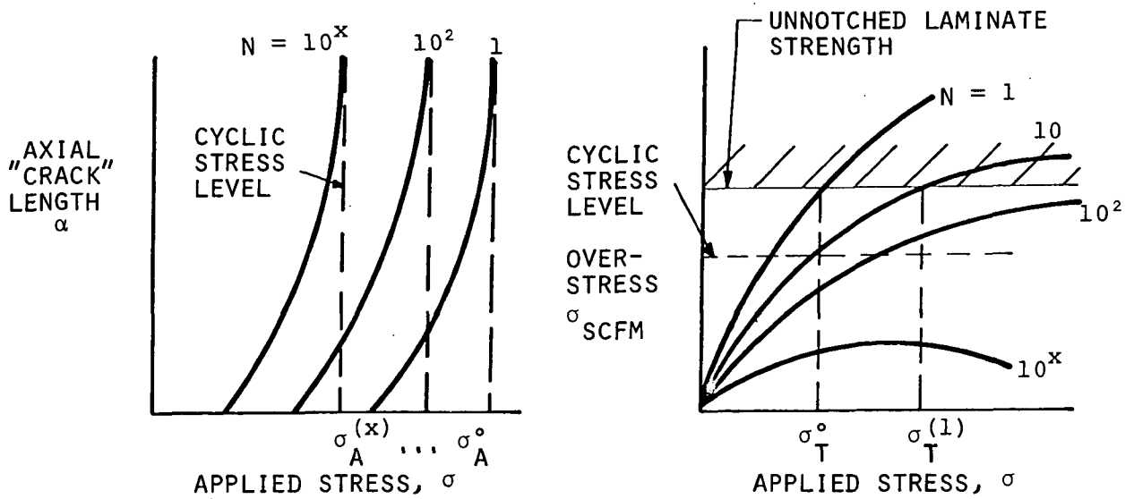
FIGURE 12. SCHEMATIC DIAGRAM OF METHOD FOR DETERMINING FATIGUE LIFETIME, RESIDUAL STRENGTH, AND AXIAL "CRACK" GROWTH OF NOTCHED LAMINATE.
