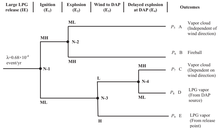
Fig. 7. Event tree with fuzzy linguistic grades.
