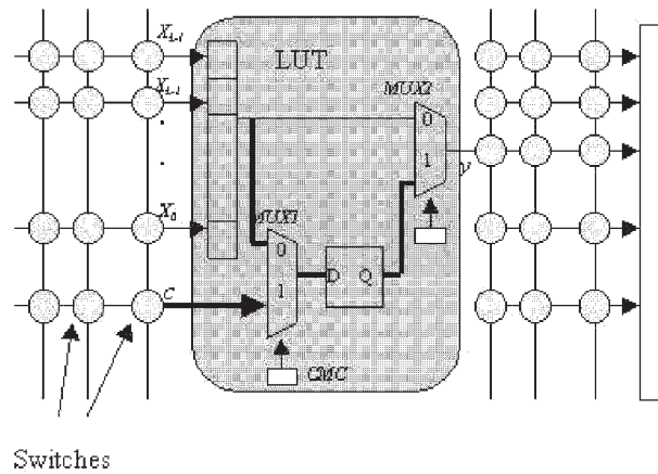
FIGURE 2 The structure of a CLB.
