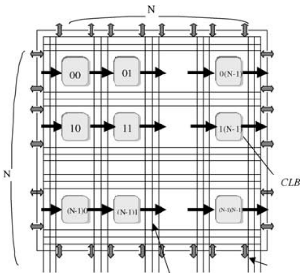
FIGURE 4 A N \times N array of CLBs.
