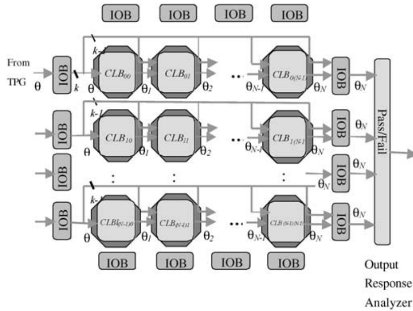
FIGURE 8 Application of test patterns.
