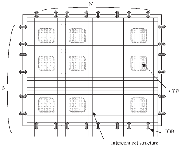
FIGURE 1 FPGA architecture.
