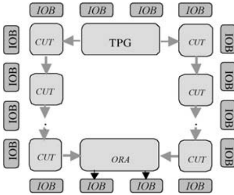
FIGURE 10 Second BIST session.
