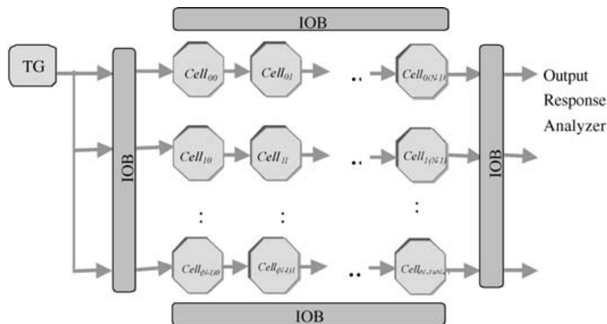
FIGURE 6 The connection structure during testing.
