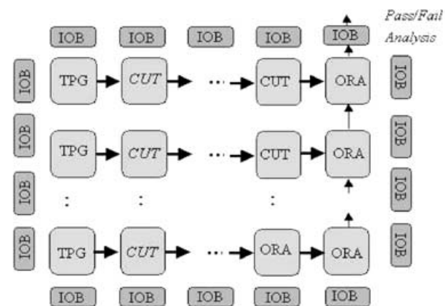
FIGURE 9 BIST structure for a BIST session.
