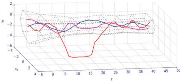
Figure 3. Basic idea of fault detection using sets (Stoican, 2011).
