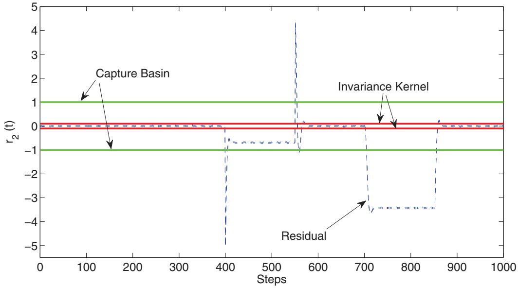
Figure 9. Invariance kernel and capture basin for second residual signal.
