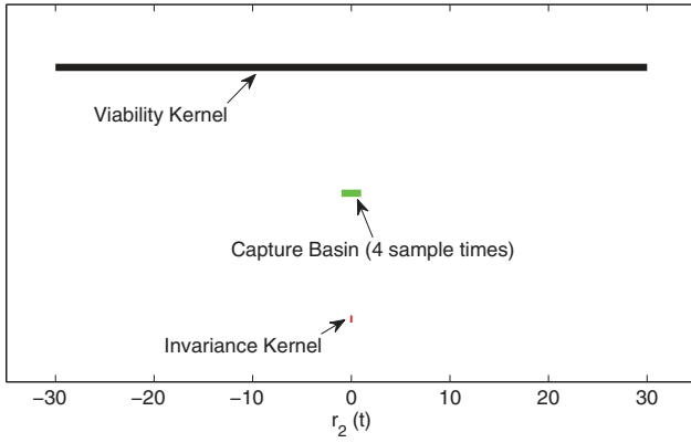
Figure 6. Kernels for residual signal r_2(t) in healthy mode.
