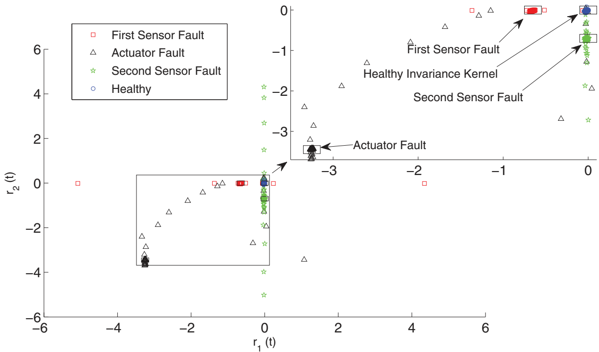
Figure 10. Invariance kernels for fault isolation.
