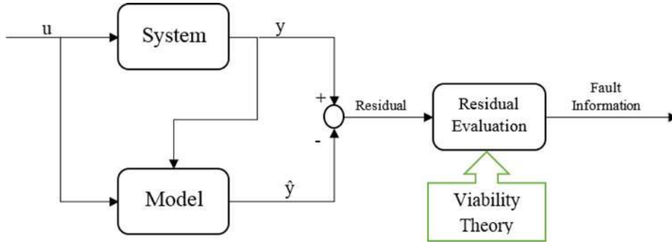
Figure 4. A general fault detection scheme.
