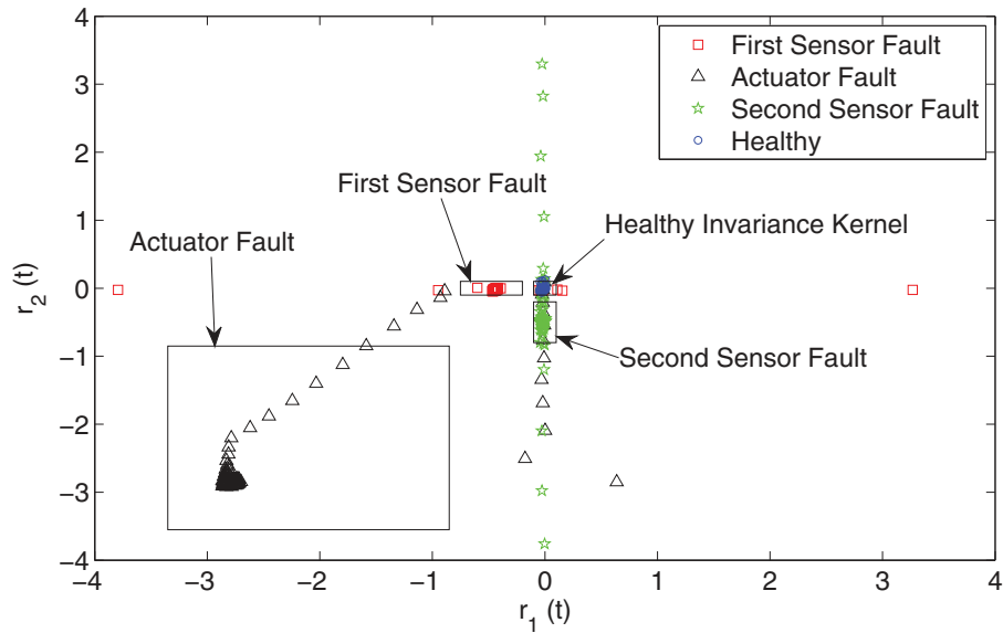
Figure 11. Invariance kernels for different interval faults.
