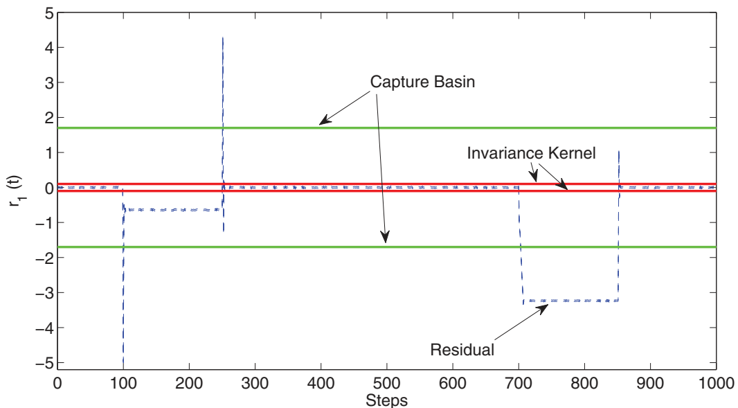
Figure 8. Invariance kernel and capture basin for first residual signal.
