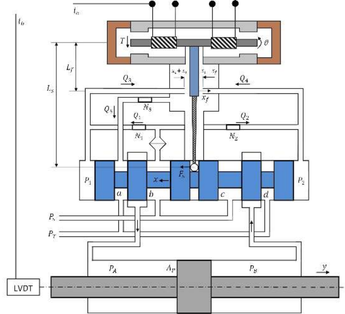
Figure 1. Functional schematic of the electro-hydraulic servo system [18]
