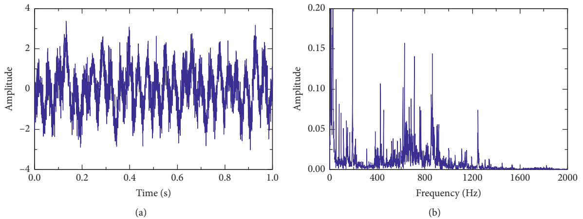
FIGURE 18: Waveform and amplitude spectrum of the outer race defect signal: (a) time-domain waveform; (b) amplitude spectrum.
