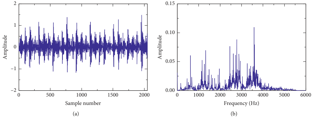
FIGURE 12: Waveform and amplitude spectrum of the inner race defect signal: (a) time-domain waveform; (b) amplitude spectrum.
