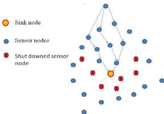
Figure 4. Routing paths when some hubs not functioning in a WSN
