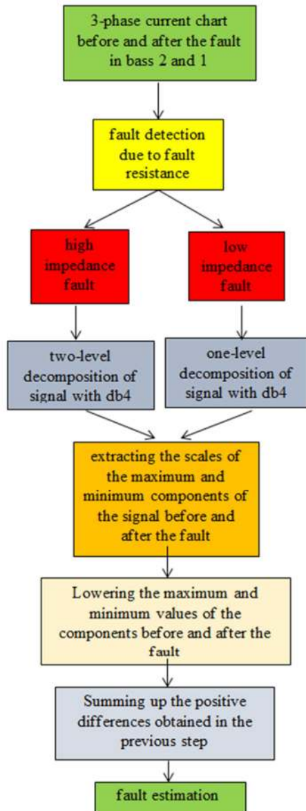
Figure 11. Current Chart of the Proposed Locator Algorithm.
