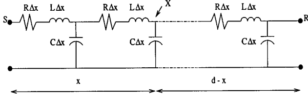
Fig. 1. Unfaulted long transmission line.
