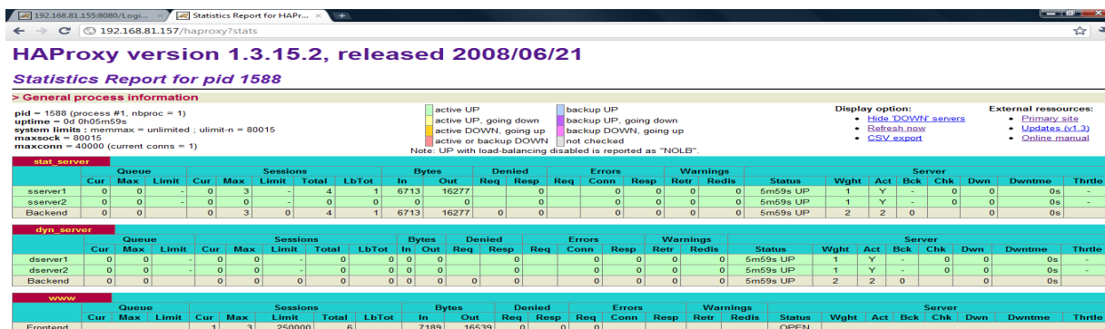
Figure 2: HAProxy Statistics
