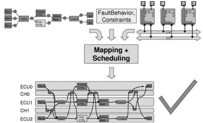
Fig. 2. SCRAPE interactive design flow.
