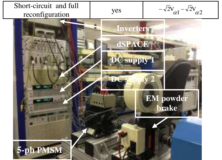
Fig. 6: Experimental platform.
