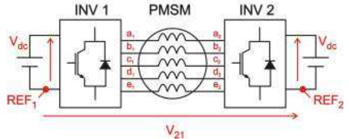
Fig. 1: Drive topology
