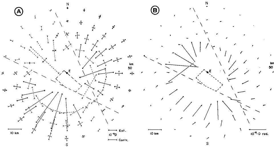
FIG. 9. (A) Computed principal strains within 50 km from a fault model with constant dislocation. (B) Computed maximum tilts within 50 km from a fault model with constant dislocation.
