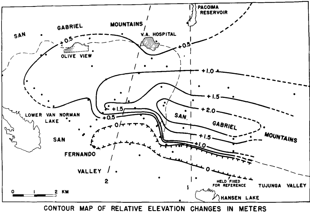
FIG. 3. Vertical displacements (relative elevation changes in meters) for part of the area surrounding the surface ruptures (Savage et al. , 1972; reproduction permitted by Dr. J. C. Savage).
